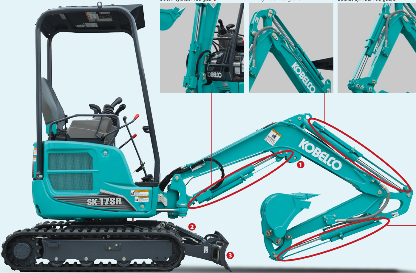
Boom cylinder rod guard
