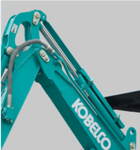
Arm cylinder rod guard
